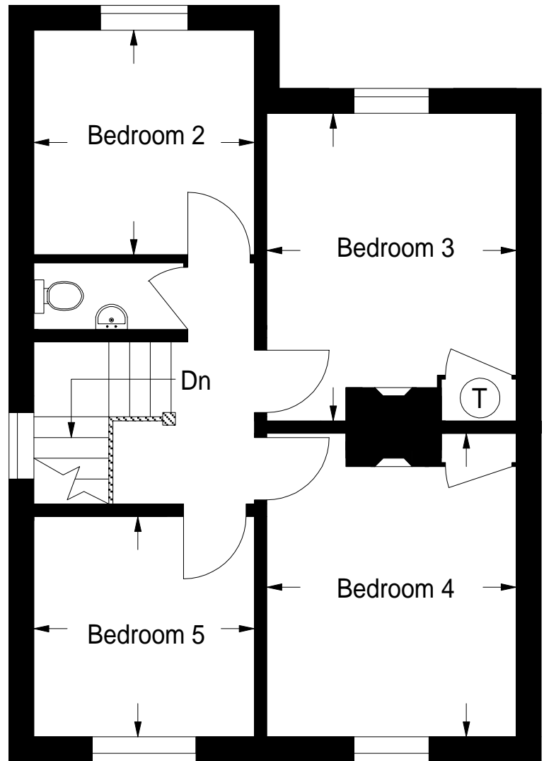
First Floor
